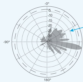
3.5 GHz Pattern
