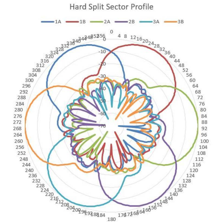
Comparison of antenna profile shows improved sidelobe suppression for each configuration profile
