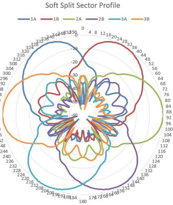
Comparison of antenna profile shows improved sidelobe suppression for each configuration profile
