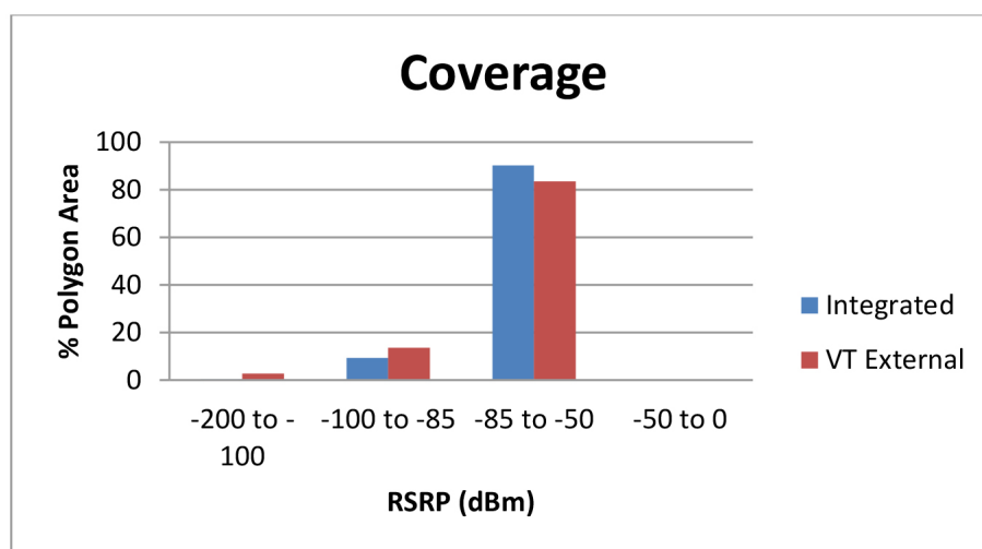
Graph 1 – Coverage Comparison
