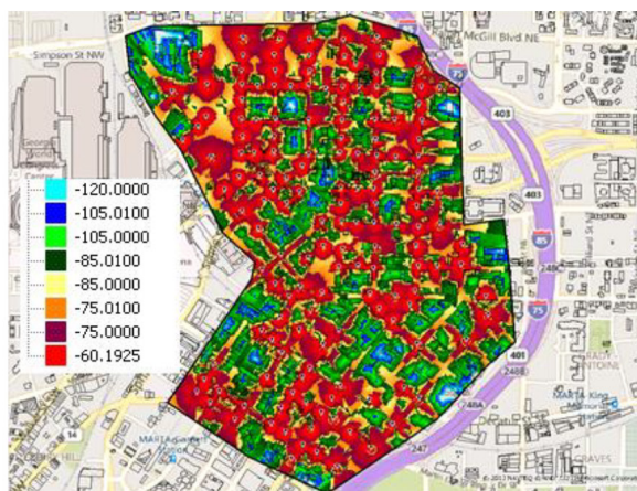
Fig 9 – VT External Antenna Coverage (dBm)
