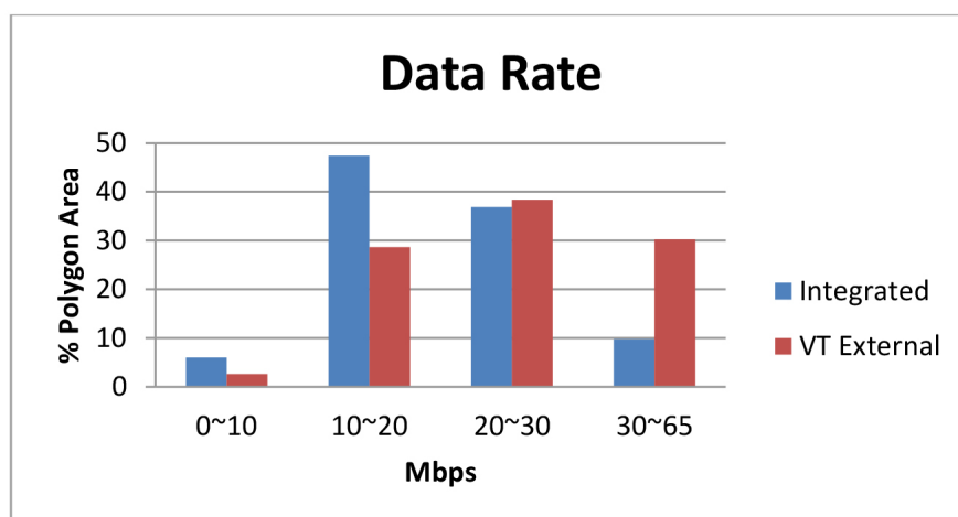
Graph 3 – Data Rate Comparison
