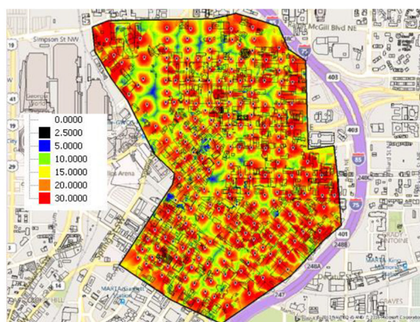
Fig 6 – Internal Antenna Data Rate (Mbps)
