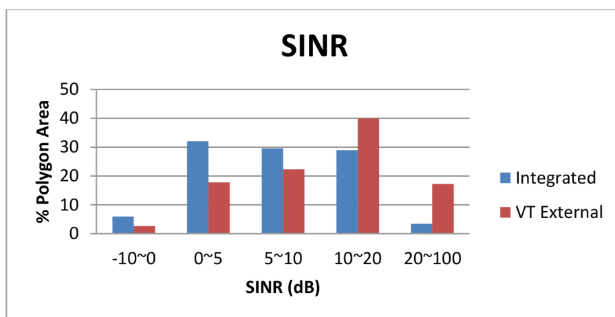
Graph 2 – SINR Comparison
